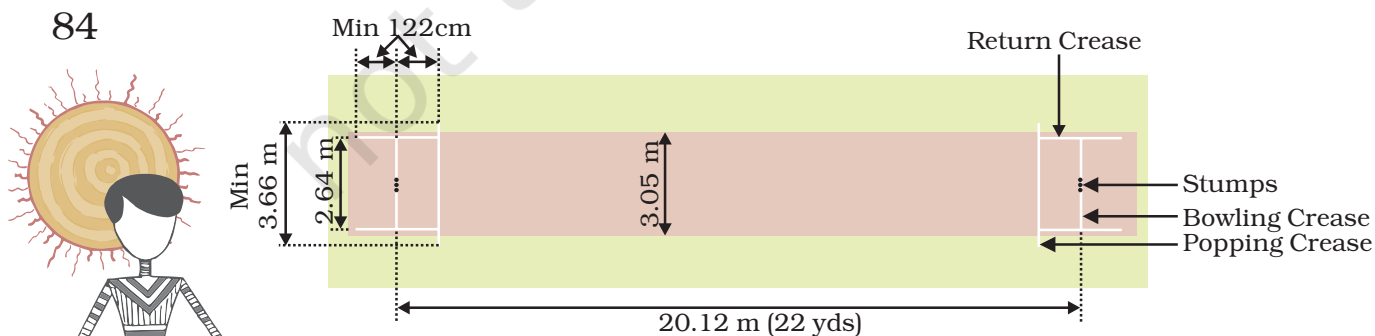
Fig. 6.8: Specifications of cricket ground
