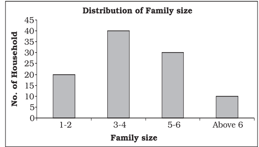
Fig. 8.2: Bar diagram
