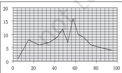
Fig. 3.2: Frequency Curve
